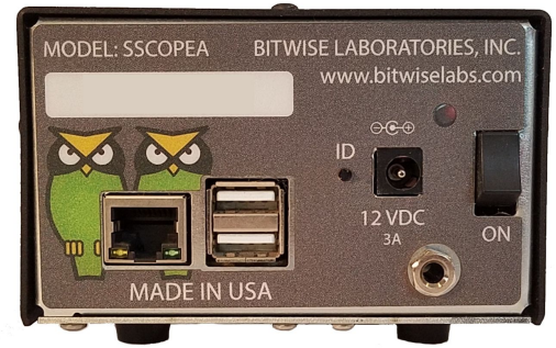
BitWise STEPScope™ Rear Panel
